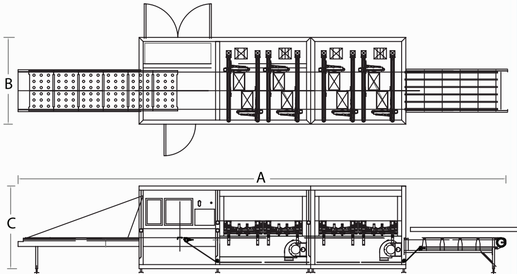
OUTFEED END
